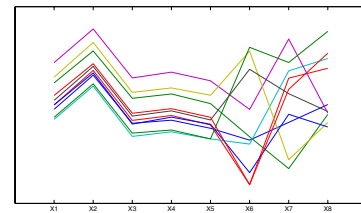
Figure 1. A shift pattern embedded in a 5-dimensional subspace
